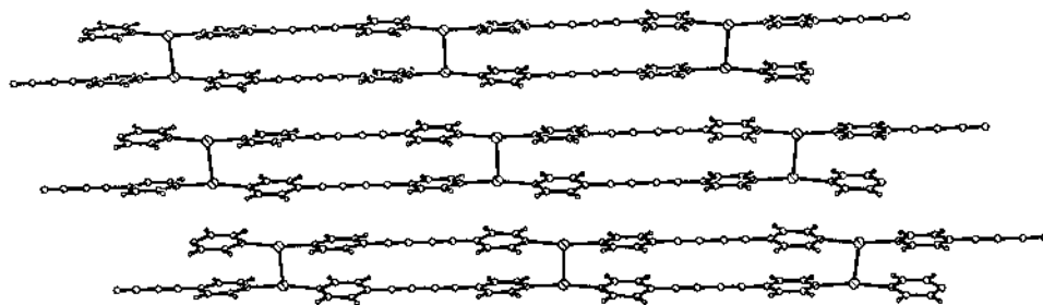
Fig. 12. View of the pairs of linear chains observed in \{[Ag(pybut)]PO_2F_2\}_\infty , in which the ligands form \pi-\pi interactions of 3.394 Å and relatively short Ag\cdots Ag interactions of 3.1929(10) Å.
