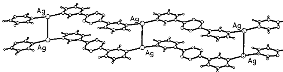
Fig. 14. View of the pairs of linear chains formed by \{[Ag(3-pytz)]CF_3SO_3\}_\infty , [ Ag\cdots Ag = 3.2199(13) Å].
