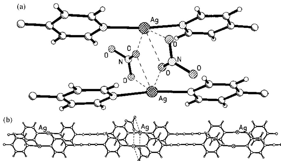
Fig. 19. (a) View illustrating the role of the weak interactions between Ag(I) ions and NO 3 - anions in \{[Ag(pybut)NO_3]\}_\infty leading to (b) staggered pairs of chains of \{[Ag(pybut)NO_3]\}_\infty .
