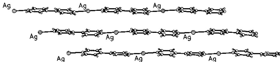
Fig. 11. View of the staggered \{[Ag(4,4'\text{-bipy})]BF_4\}_\infty chains, minimising Ag\cdots Ag contacts and \pi\text{-}\pi interactions between adjacent chains.
