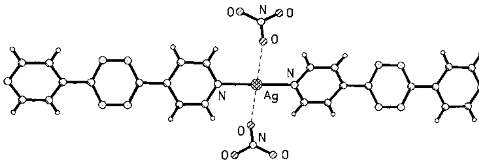
Fig. 16. View of the pseudo-square planar geometry of the Ag(I) ion in \{[Ag(4\text{-pytz})]NO_3\}_\infty .
