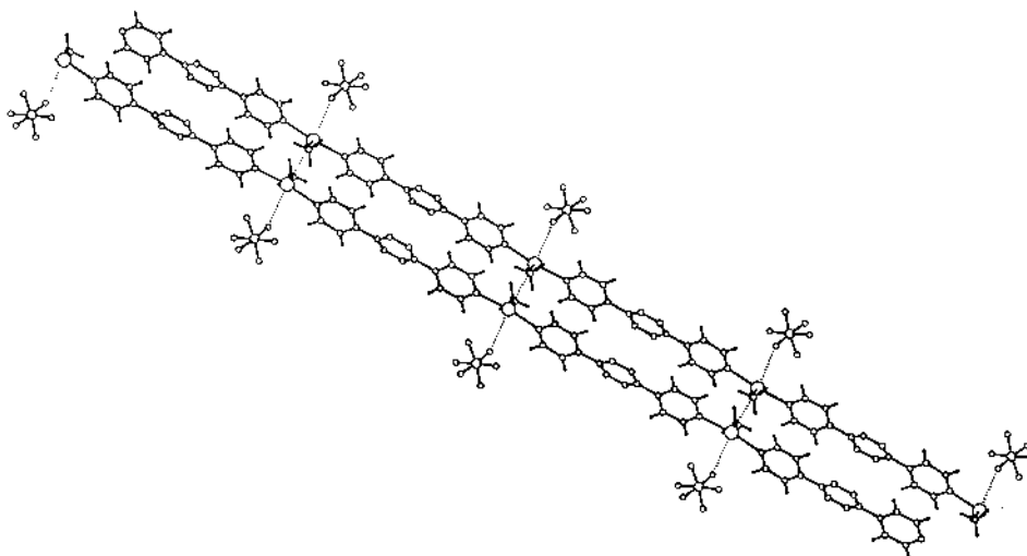
Fig. 13. View of the pairs of linear chains formed by \{[Ag(4-pytz)]X\}_\infty ( X = BF_4^-, PF_6^- ). ( Ag\cdots Ag = 3.312(1) Å ( BF_4^- ), 3.230(1) Å ( PF_6^- )) (reproduced with permission from Ref. [14]).
