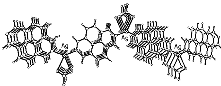
Fig. 20. View of the undulating chains of \{[Ag(diaz)NO_3]\}_\infty which stack to give a two-dimensional sheet through \pi - \pi interactions (3.339 Å).
