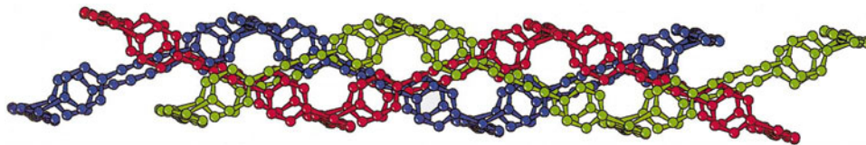
Fig. 8. View of \{[\text{Cu}_2(\text{MeCN})_2(\text{pybut})_3](\text{PF}_6)_2\}_\infty showing the undulating nature of the ladders which allows them to interweave in a parallel fashion (reproduced with permission from Ref. [11]).
