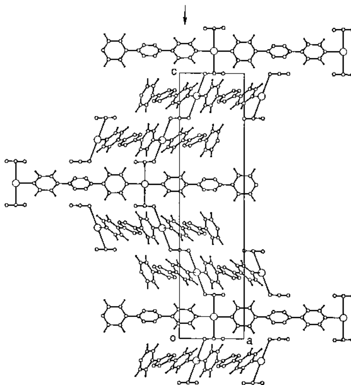
Fig. 17. View of the helical staircase motif formed by \{[Ag(4\text{-pytz})]NO_3\}_\infty (reproduced with permission from Ref. [14]).
