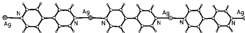
Fig. 10. View of the linear chains formed by \{[Ag(4,4'\text{-bipy})]BF_4\}_\infty .
